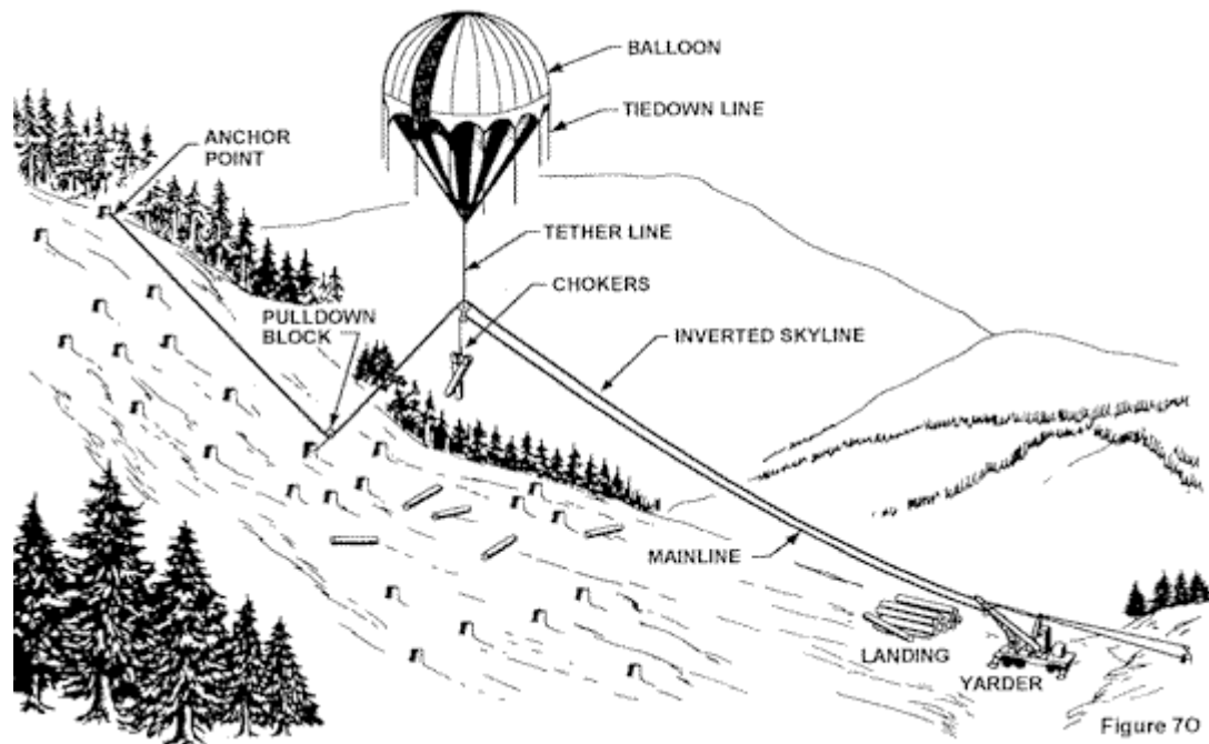
Figure 7. Balloon Extraction – Haulback Configuration. Picture from [9].
