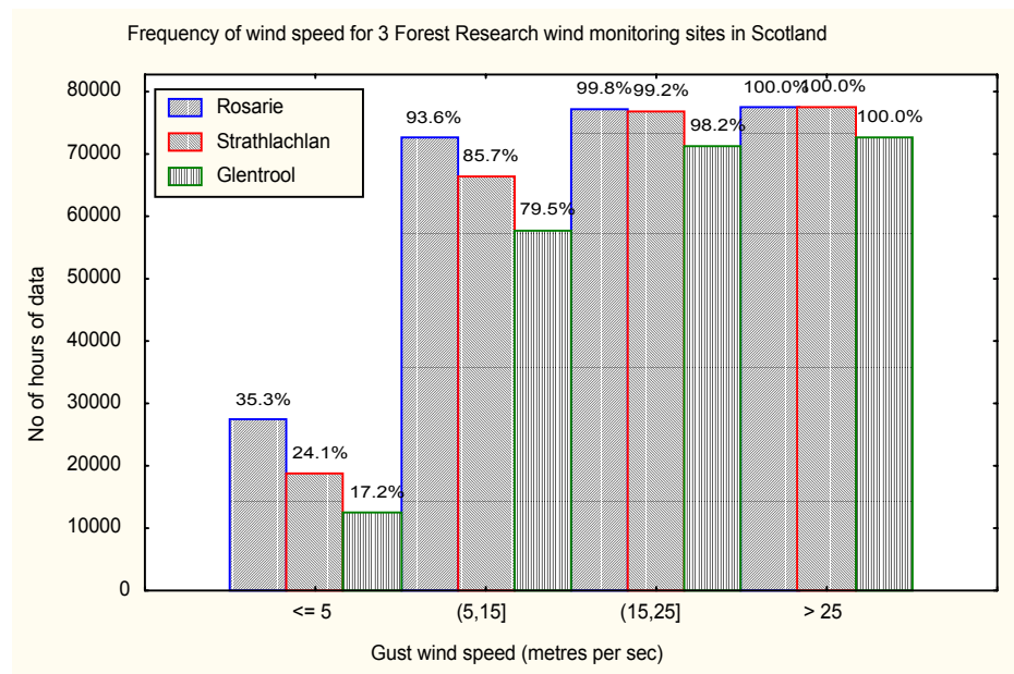
Figure 8. Cumulative frequency of hours with gust wind speeds measured at 10m above the ground on an open site. Rosarie – 320m hill top near Elgin, Strathlachlan – 370 m hill top near Strachur, Glentool – 420m hill top near Barrhill.
