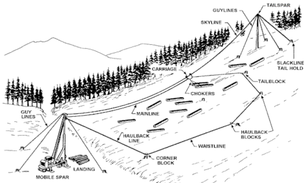
Figure 6. Example of a slack line system used in Scotland. Picture from [9].
