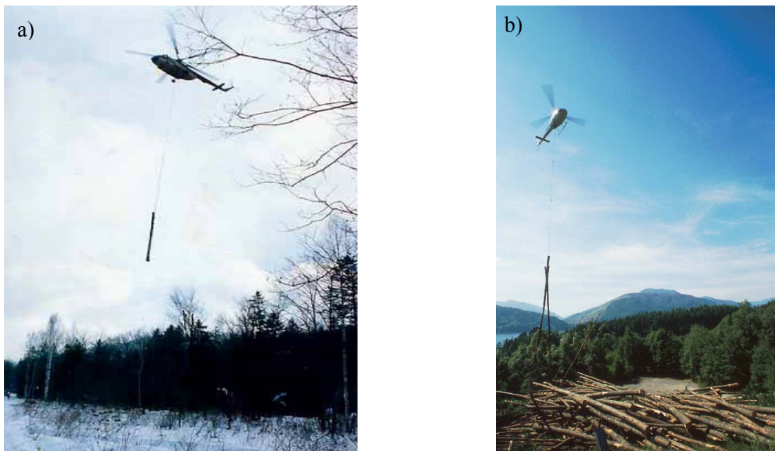
Figure 5. Helicopter extraction a) in Russia [1] and b) in the UK [11].
